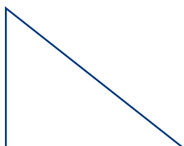
Triangle obtusangle
